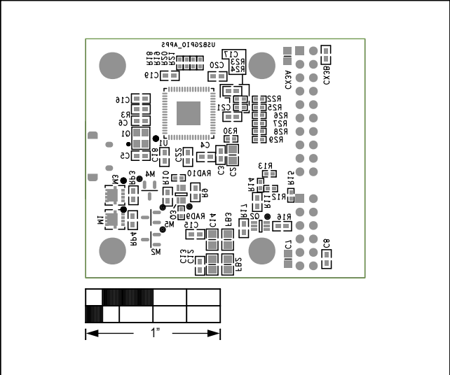
USB2GPIO# Adapter Board—Bottom Silkscreen
