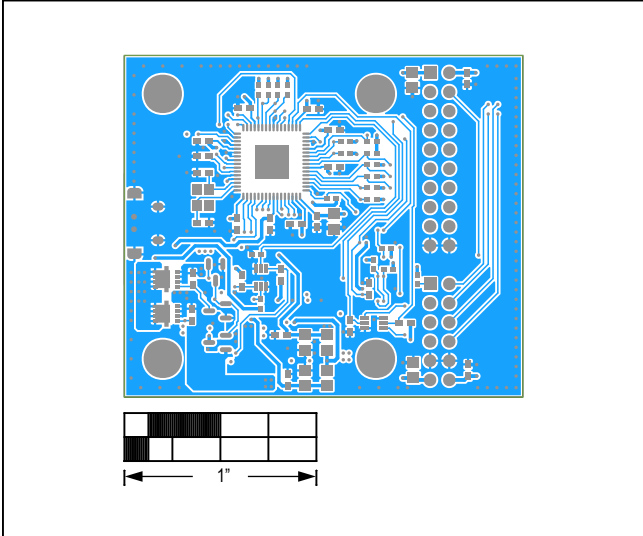
USB2GPIO# Adapter Board—Bottom
