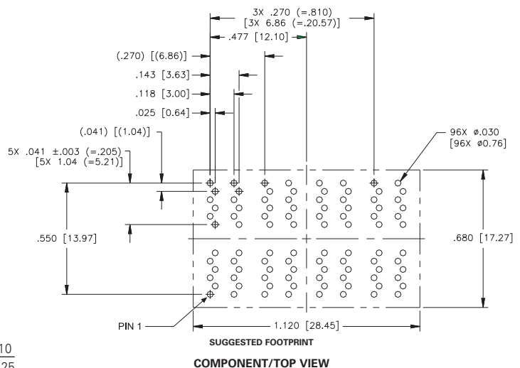
SUGGESTED FOOTPRINT COMPONENT/TOP VIEW
