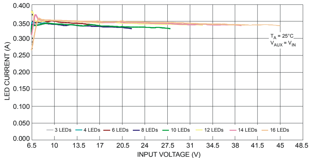
Figure 15 I_{\text{LED}} vs. Input Voltage & Number of LED
