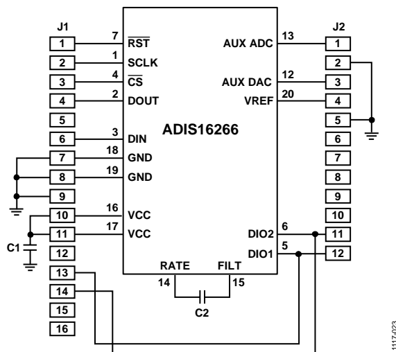
Figure 22. Electrical Schematic
