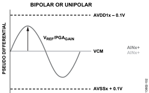
Figure 102. Σ-Δ ADC Input Signal Configuration, Pseudo Differential
