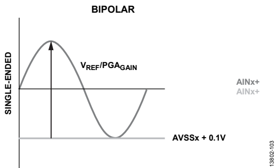
Figure 103. Σ-Δ ADC Input Signal Configuration, Single-Ended Bipolar
