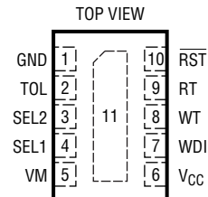
DDB PACKAGE 10-LEAD (3mm x 2mm) PLASTIC DFN T_{JMAX} = 125^{\circ}\text{C} , \theta_{JA} = 43^{\circ}\text{C/W} EXPOSED PAD (PIN 11) PCB GND CONNECTION OPTIONAL LTC2917
