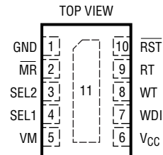
DDB PACKAGE 10-LEAD (3mm x 2mm) PLASTIC DFN T_{JMAX} = 125^{\circ}\text{C} , \theta_{JA} = 43^{\circ}\text{C/W} EXPOSED PAD (PIN 11) PCB GND CONNECTION OPTIONAL LTC2918
