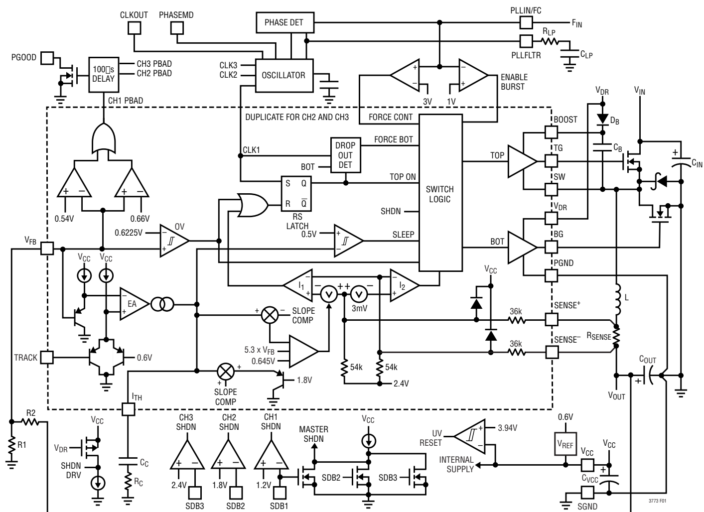
Figure 1. Functional Diagram
