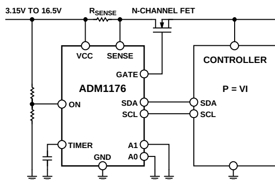
Figure 2. Applications Diagram
