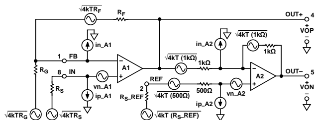
Figure 52. Noise Sources
