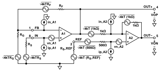
Figure 52. Noise Sources
