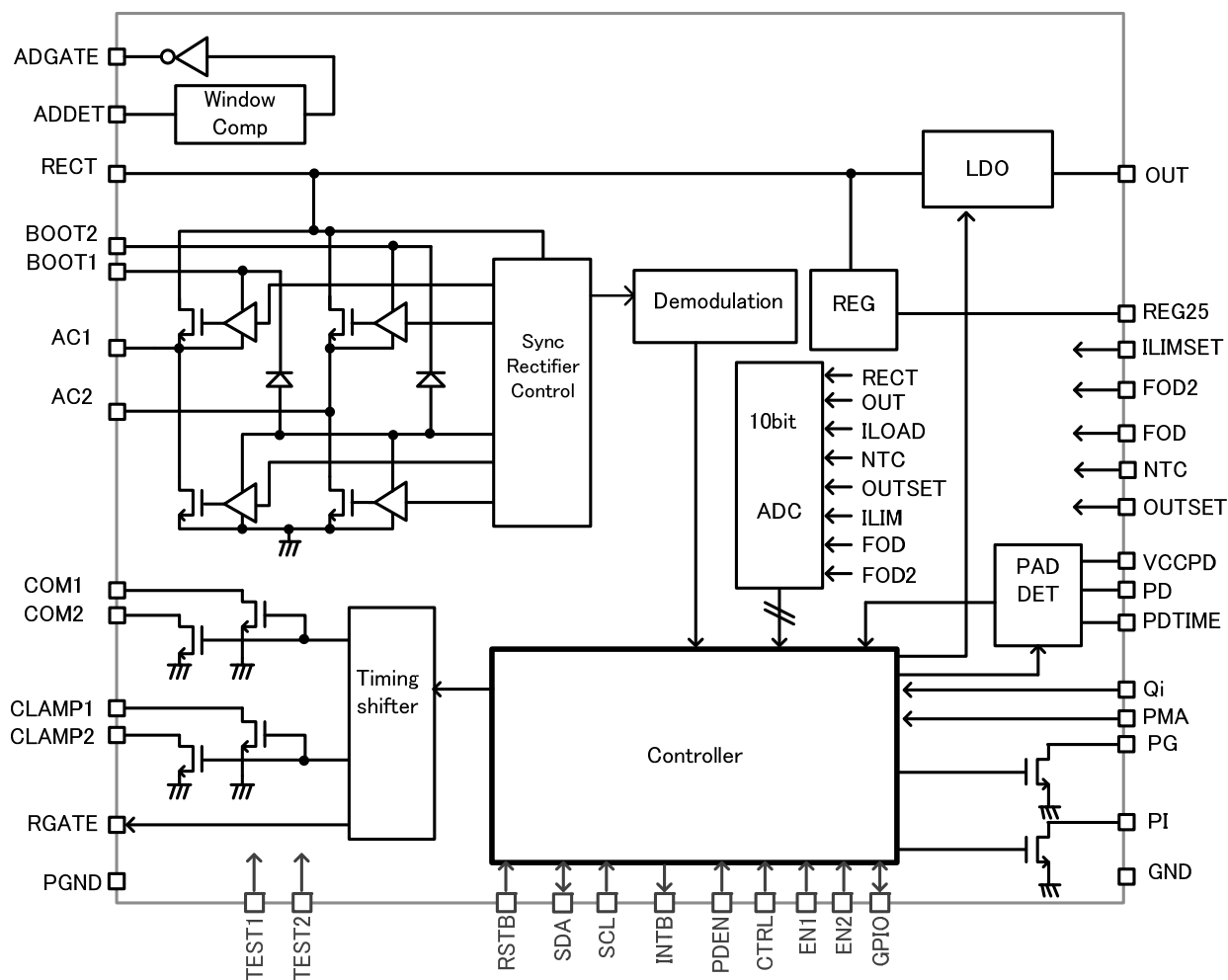
Figure 4. Block Diagram
