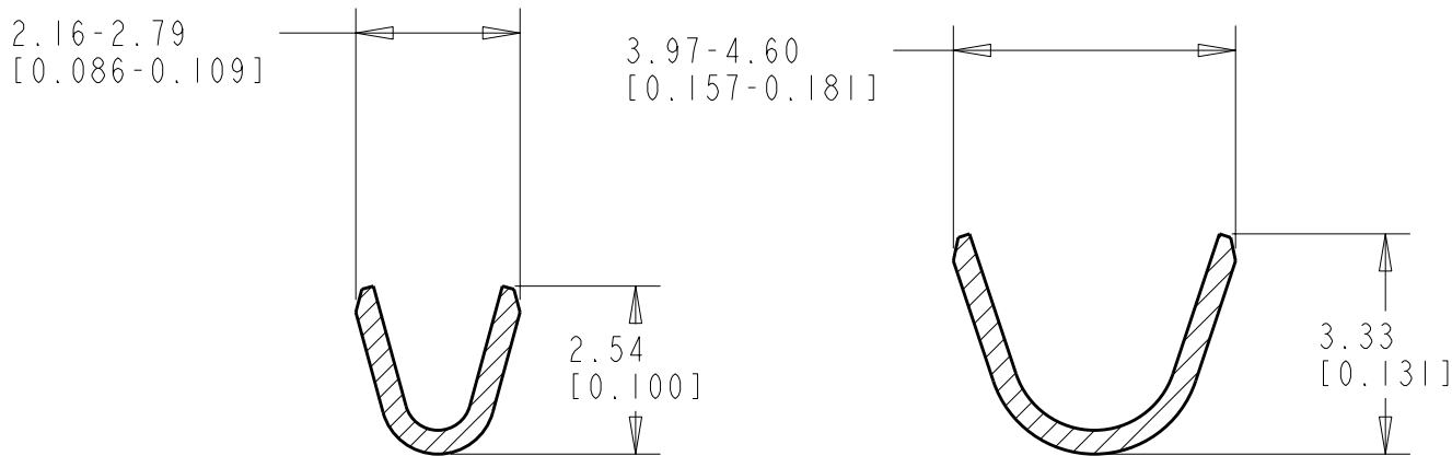
SECTION C-C
