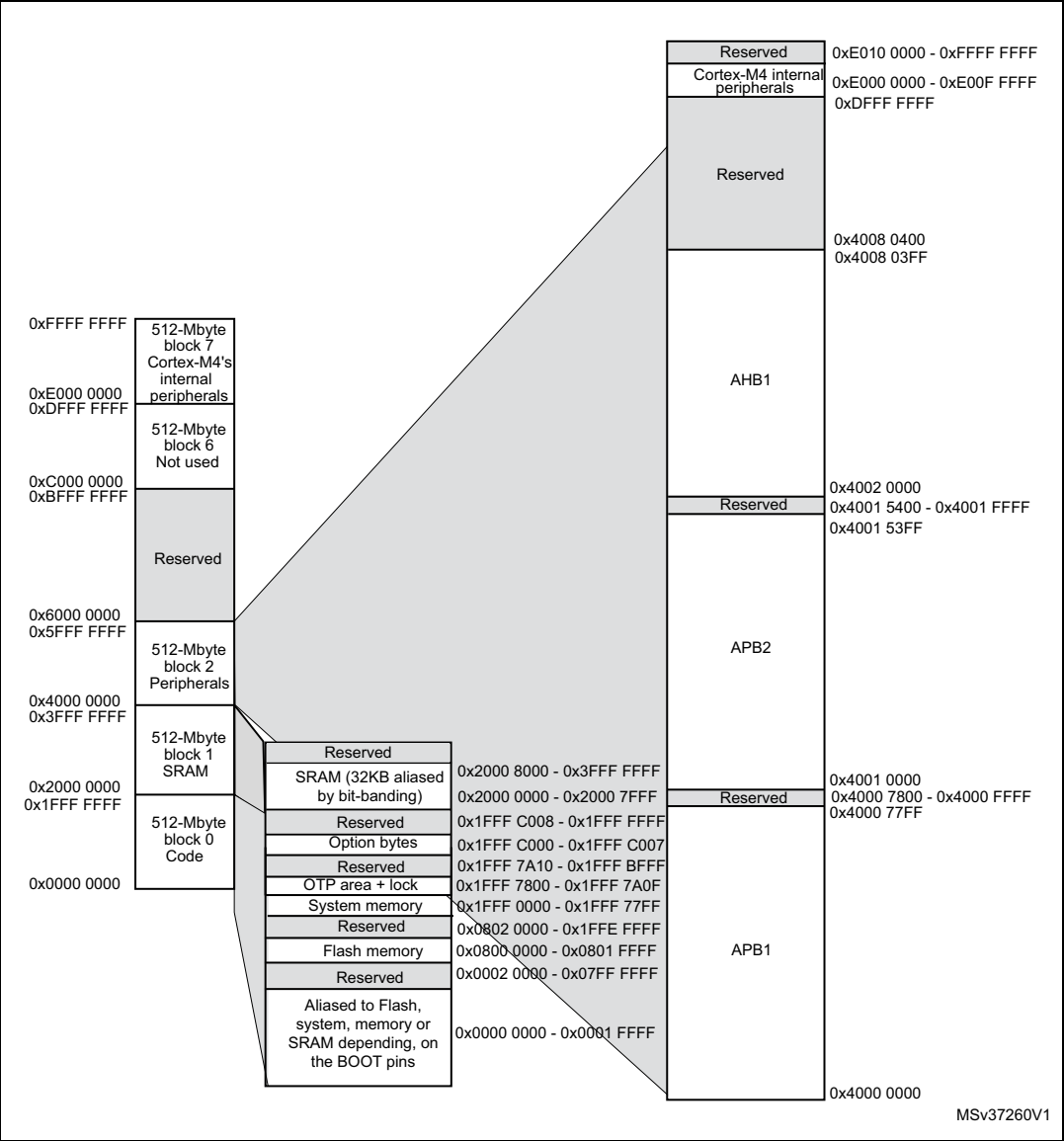
Figure 8. Memory map
