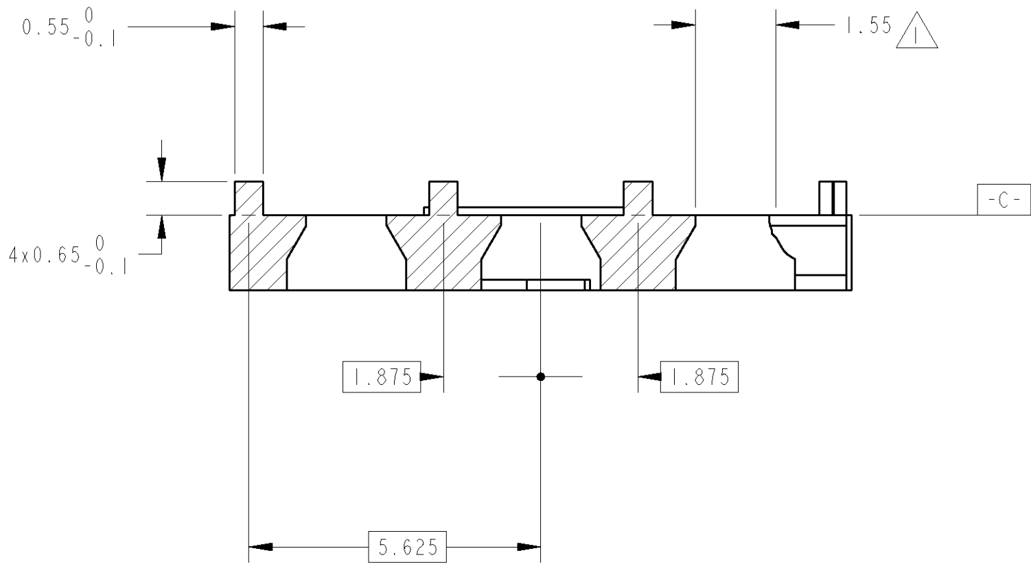
SECTION A - A SCALE 10:1
