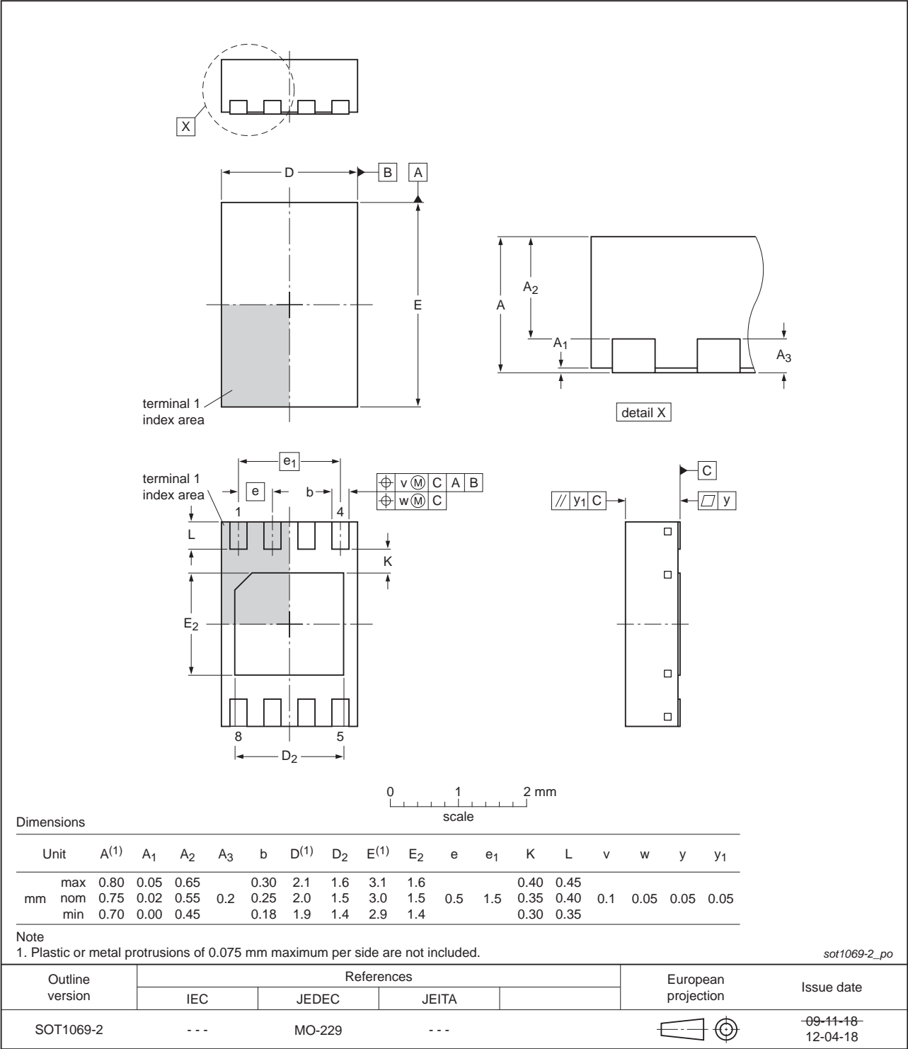
Fig 27. Package outline SOT1069-2 (HWSO8) of PCF85063TP
