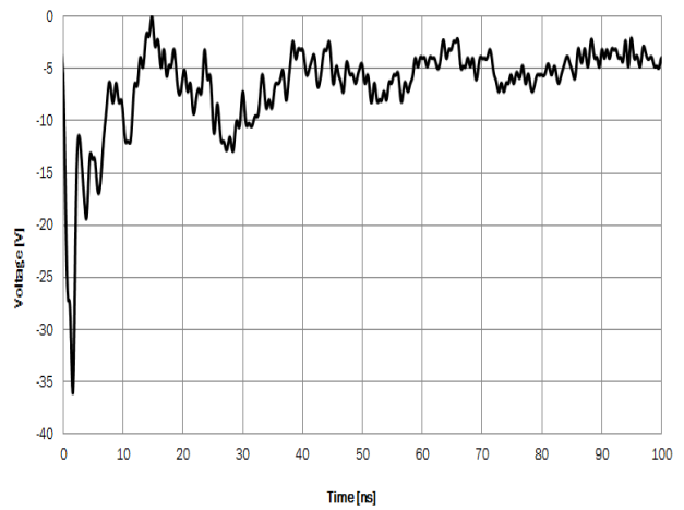
Figure 12. ESD5111 Negative 8 kV ESD Contact Discharge
