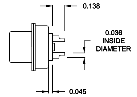
SIGNAL CONTACTS ACCEPTS UP TO 20 AWG WIRE
