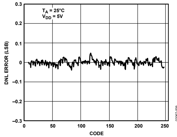
Figure 9. AD5307 DNL
