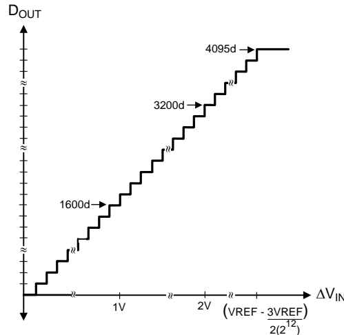
Figure 26. D_{OUT} vs \Delta V_{IN} for a 12-bit ADC assuming V_{REF} = 2.56V .
