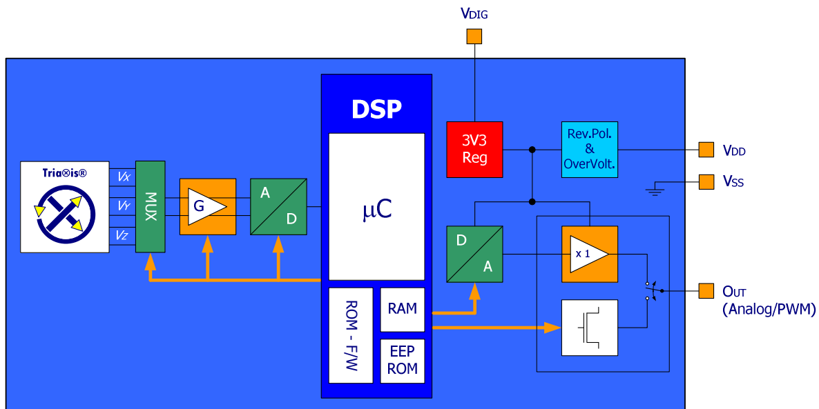
Figure 1 - MLX 90360 Block Diagram
