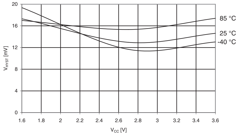
Figure 35-34. Analog Comparator Hysteresis vs. V_{CC}
