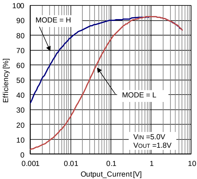
Figure 22. Efficiency vs Load Current ( V_{IN}= 5.0V , V_{OUT}= 1.8V , L= 1.5\mu H )
