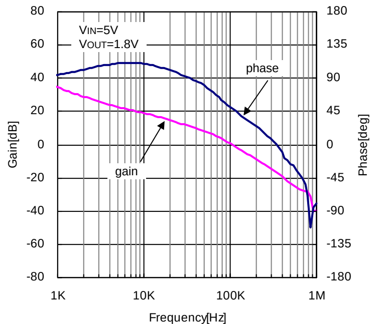
Figure 25. Closed Loop Response ( V_{IN}=5V , V_{OUT}=1.8V , I_{OUT}=6A , L=1.5\mu H , R3=6.8k\Omega , C6=5600pF , C14=100pF )
