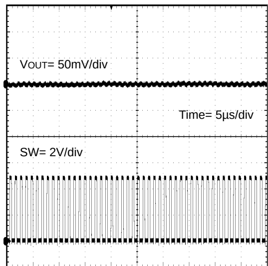
Figure 43. SW Waveform (PWM Control) ( V_{IN}=5.0V , V_{OUT}=1.8V , I_{OUT}=1A )
