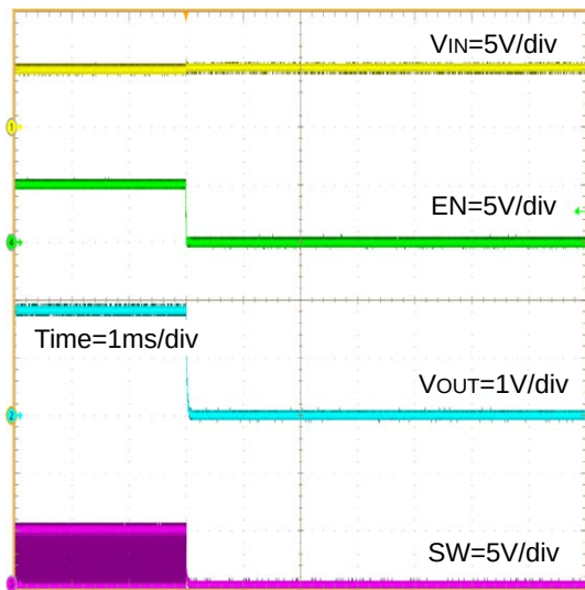
Figure 29. Power Down (EN= 5V→0V)
