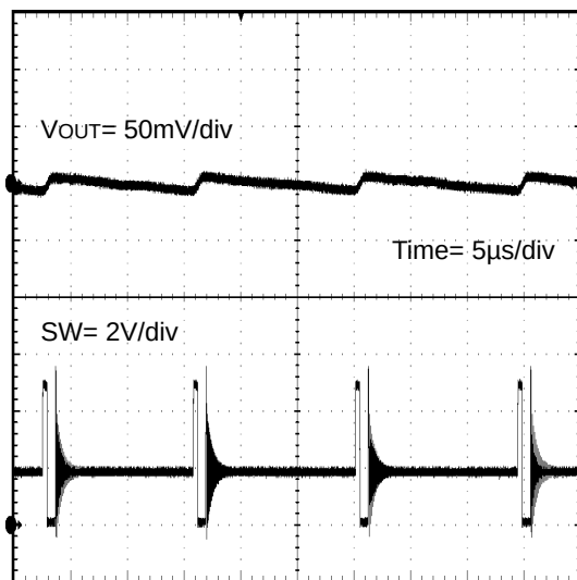
Figure 42. SW Waveform(SLLM™ Control) ( V_{IN}=5.0V , V_{OUT}=1.8V , I_{OUT}=50mA )
