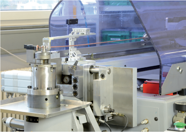
Automatic bending
