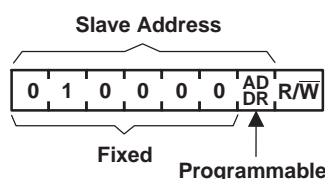
Figure 4. TCA6408A Address
