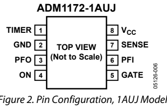
Figure 2. Pin Configuration, 1AUJ Model
