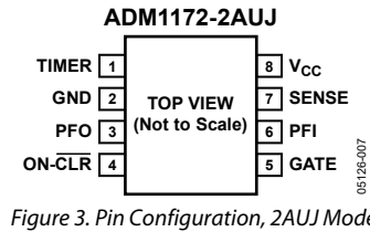
Figure 3. Pin Configuration, 2AUJ Model
