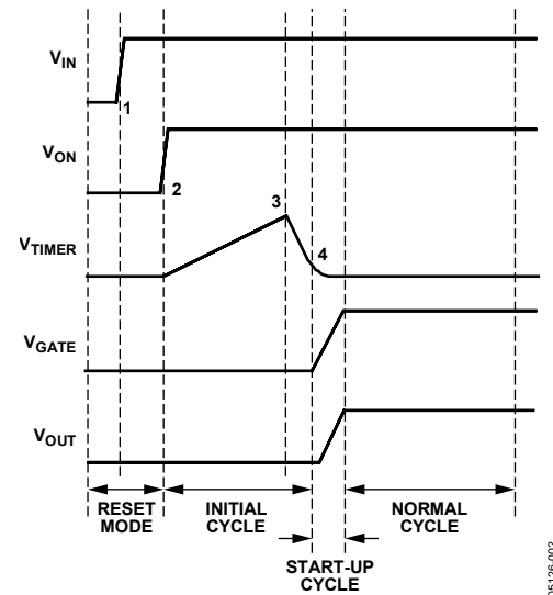
Figure 38. Power-Up Timing
