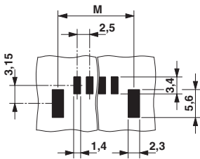
Drilling diagram
