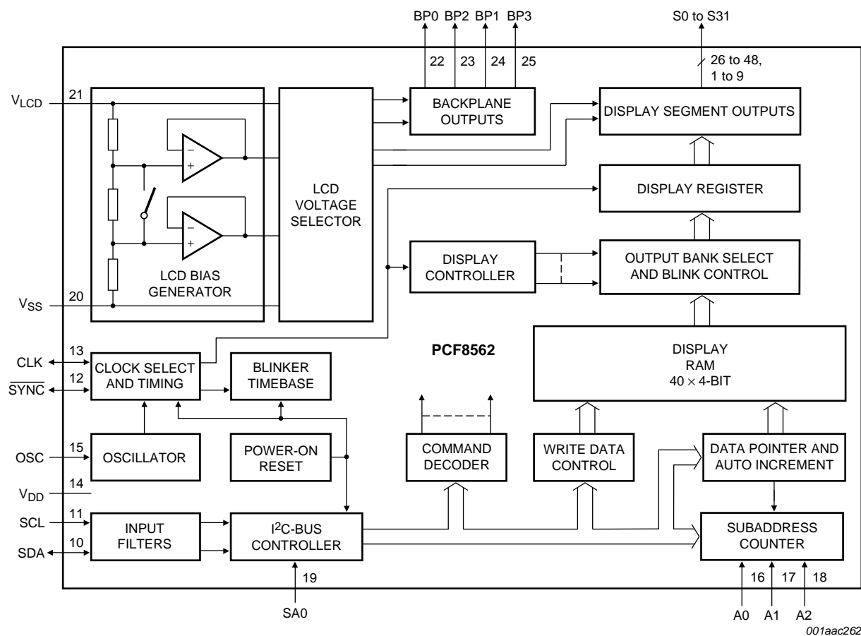
Fig 1. Block diagram of PCF8562
