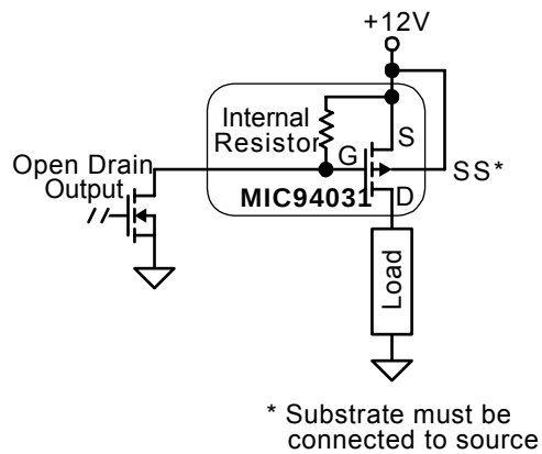
Figure 2. Power Control Application
