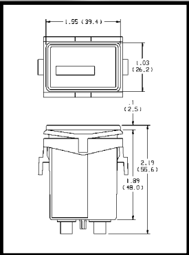
Retainer Mount: Panel cutout 1.45 x .95 rectangular opening. *
