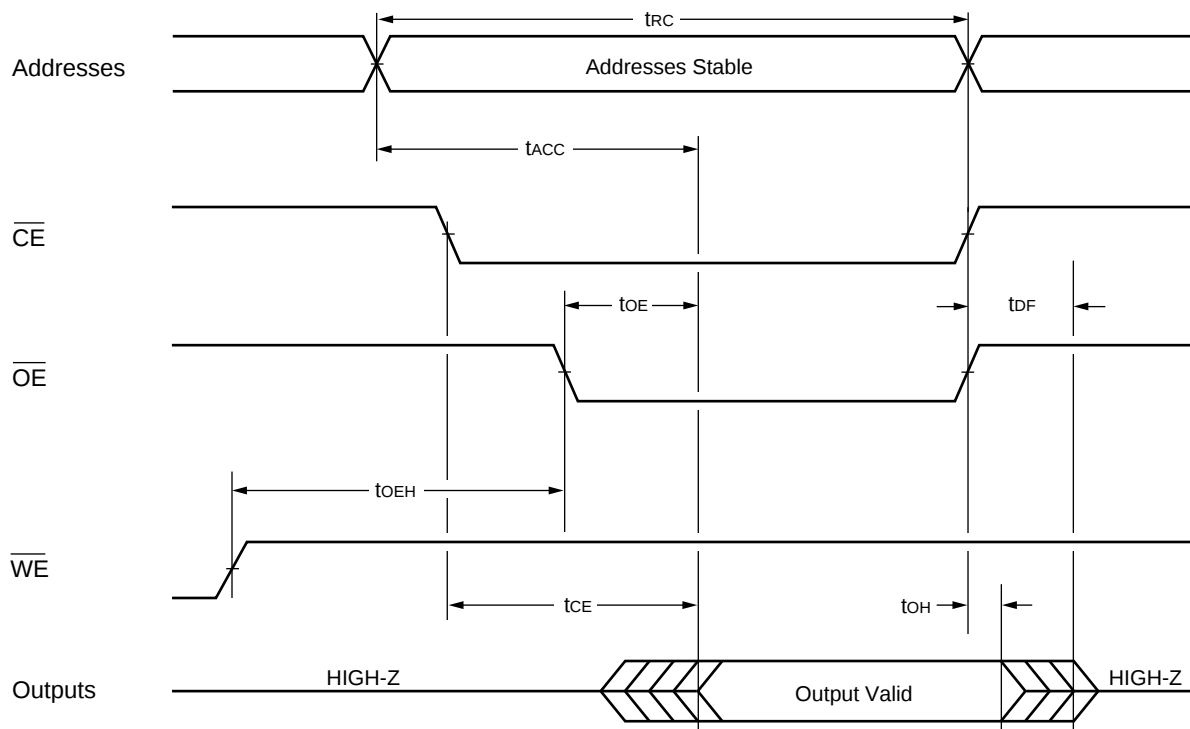
Figure 5.1 AC Waveforms Read Operations
