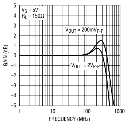
Frequency Response
