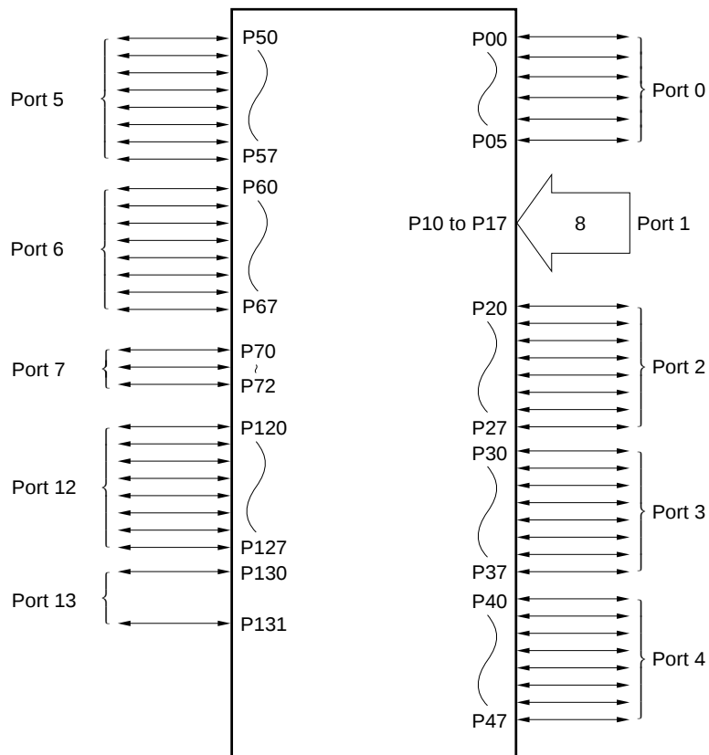
Figure 7-1. Port Configuration
