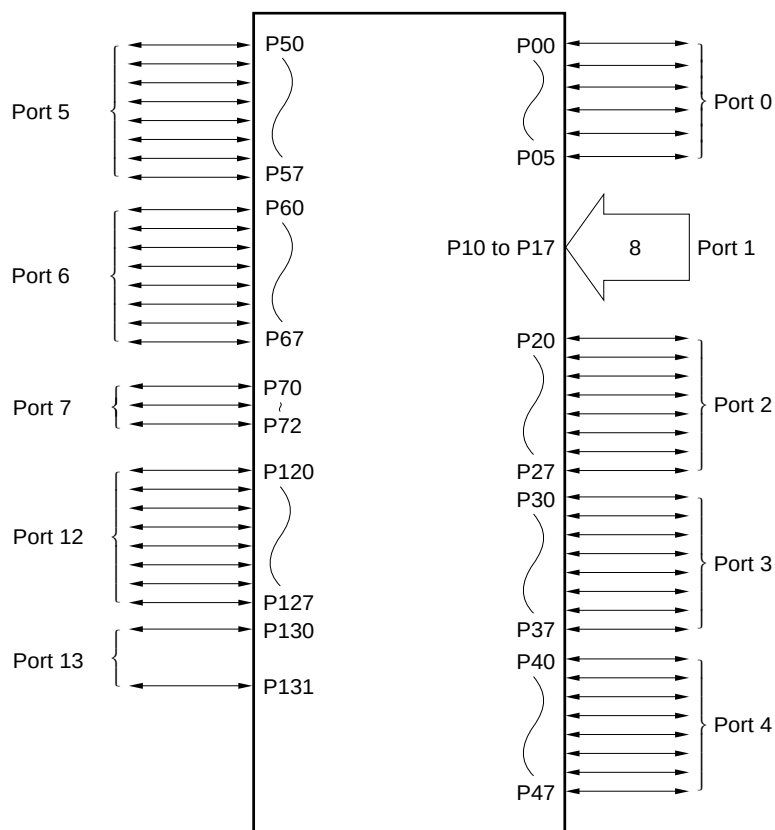
Figure 7-1. Port Configuration
