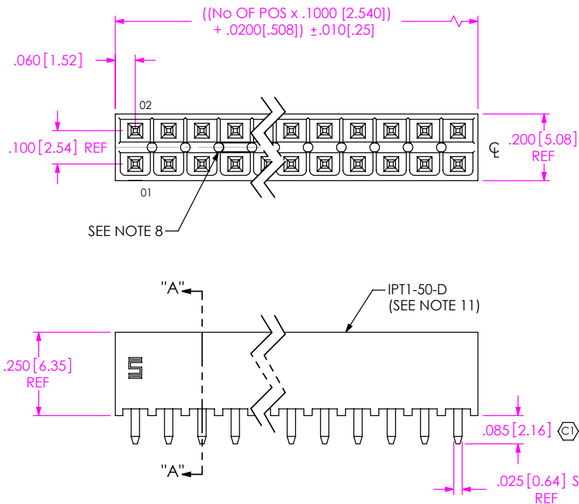
FIG 1 (IPT1-125-01-XX-D-XXX SHOWN)
