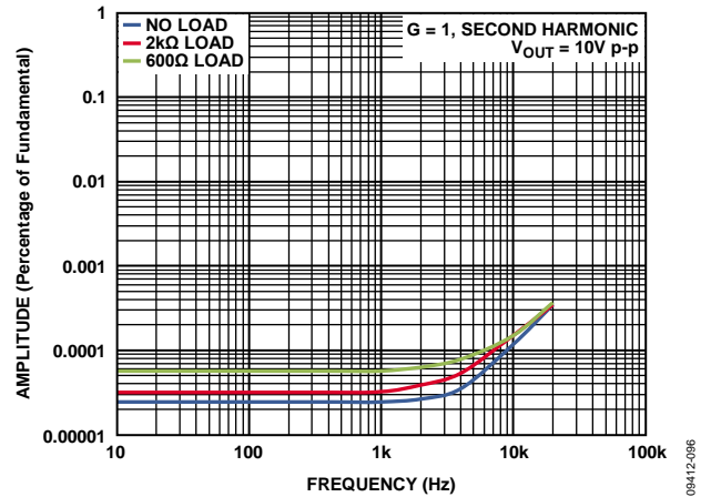
Figure 51. Second Harmonic Distortion vs. Frequency, G = 1
