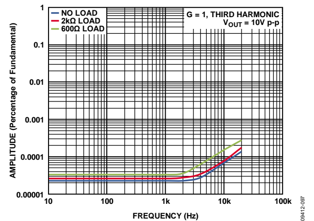
Figure 52. Third Harmonic Distortion vs. Frequency, G = 1
