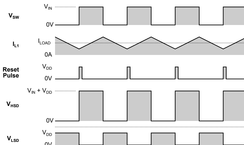
Figure 3. PWM-Mode Timing
