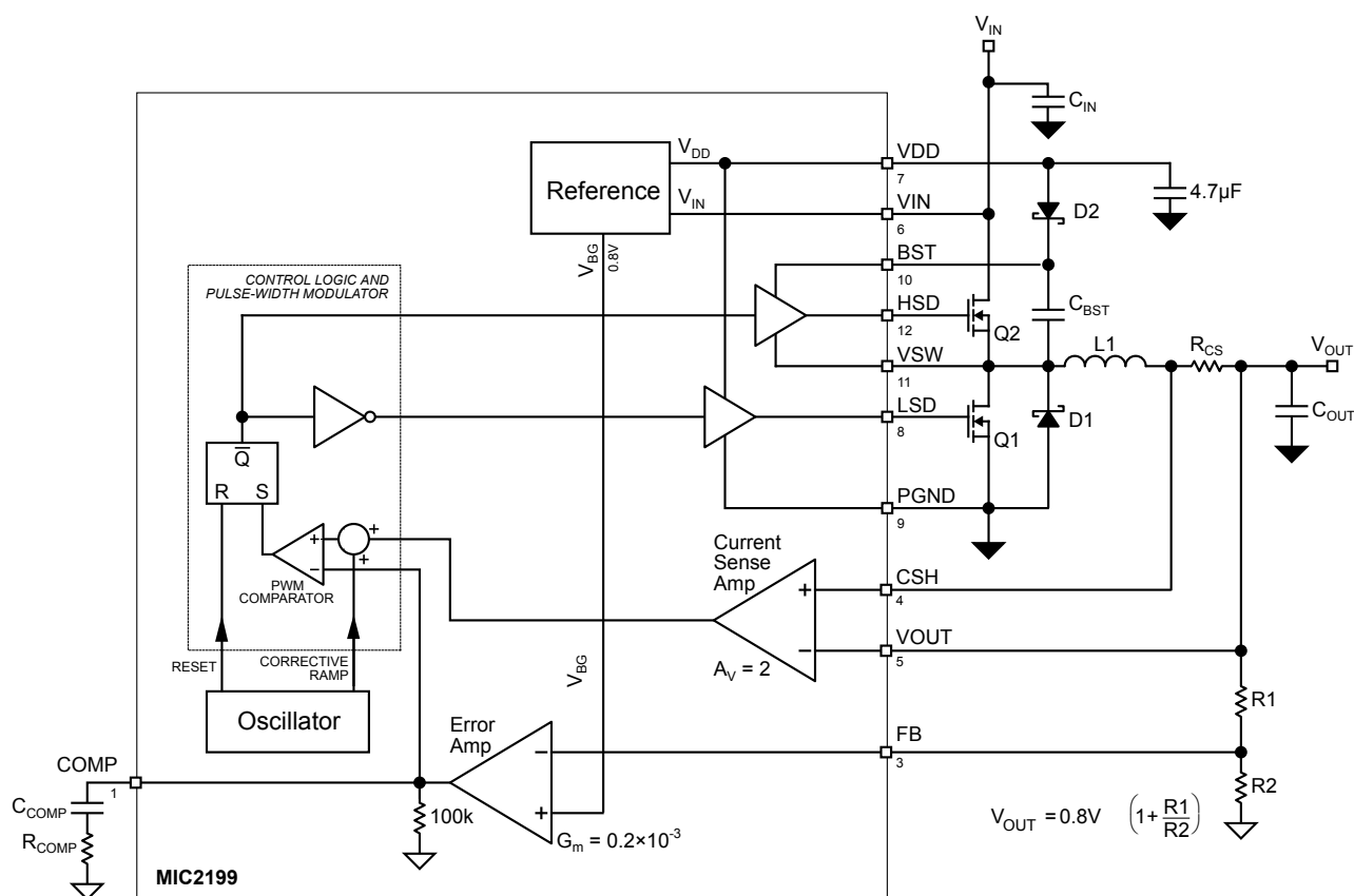
Figure 2. PWM Operation
