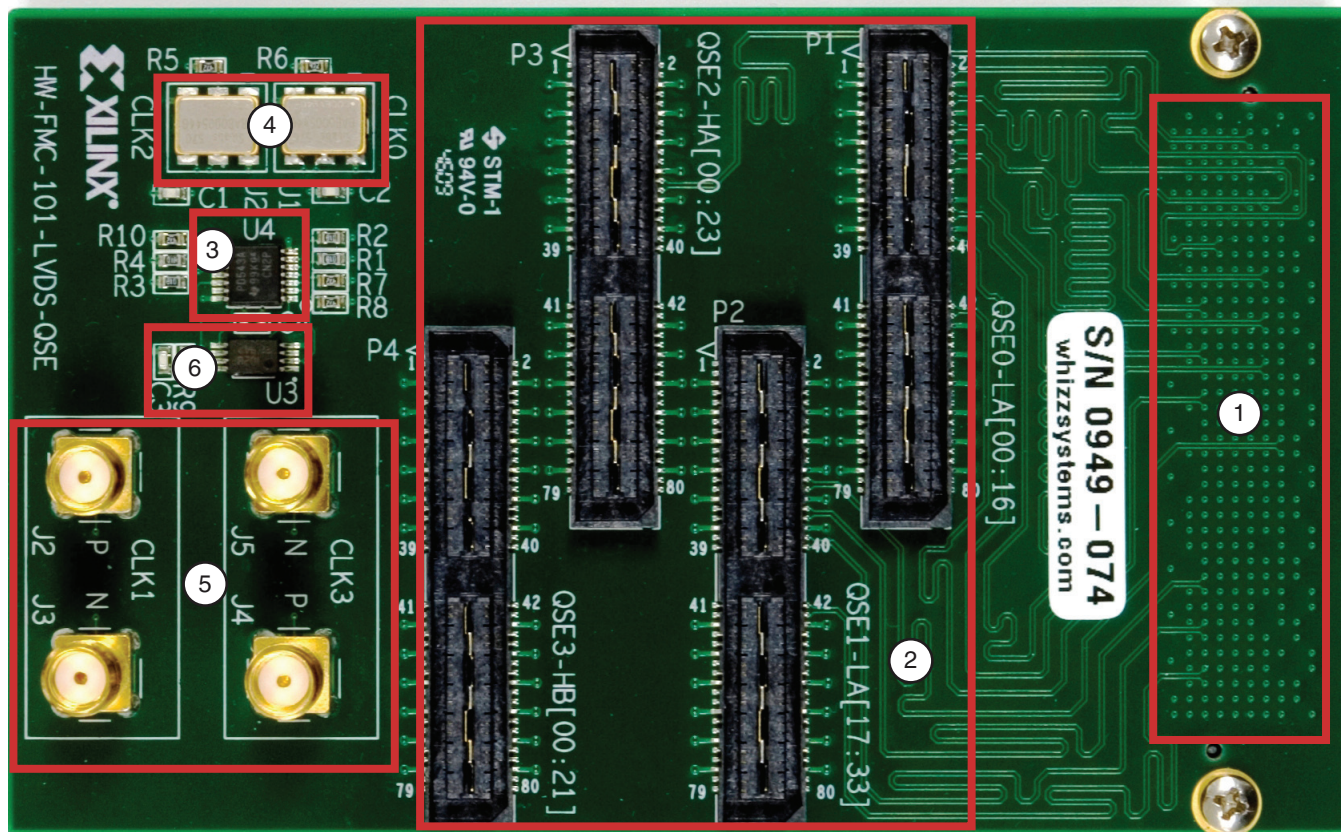
Figure 1-3: XM101 Features
