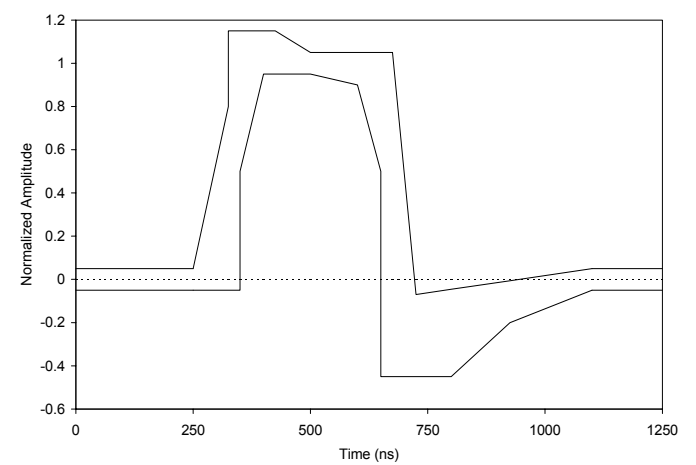
Figure 31. DSX-1 Waveform Template
