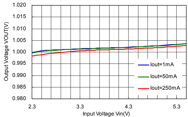
RP508K101x, V_{OUT} = 1.0\text{ V} MODE = "H" forced PWM control
