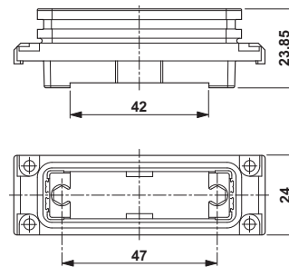
Adapter plate
