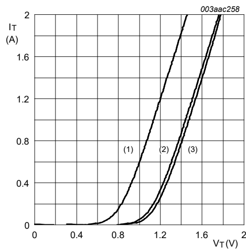
V_o = 1.13 \text{ V} R_s = 0.31 \Omega (1) T_J = 125^{\circ}\text{C} ; typical values (2) T_J = 125^{\circ}\text{C} ; maximum values (3) T_J = 25^{\circ}\text{C} ; maximum values Fig. 10. On-state current as a function of on-state voltage
