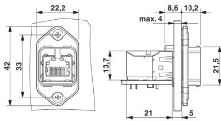
Push-Pull panel mounting frame RJ45
