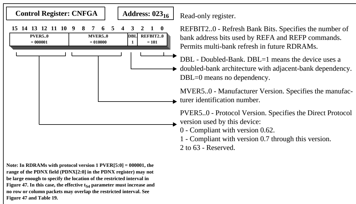
Figure 28: CNFGA Register
