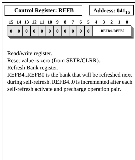
Figure 32: REFB Register
