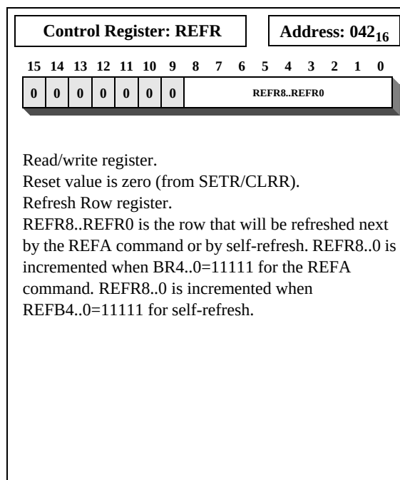
Figure 34: REFR Register
