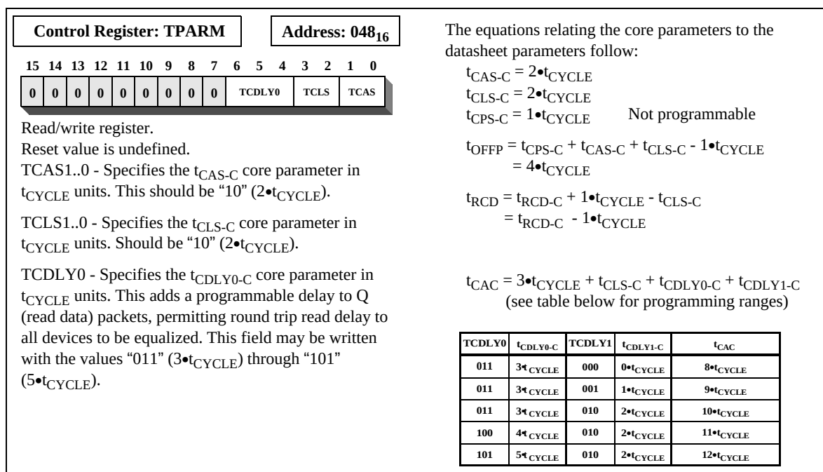
Figure 39: TPARM Register
