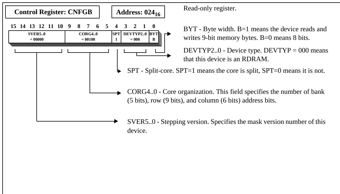
Figure 29: CNFGB Register
