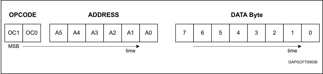
Figure 23. SDI frame
