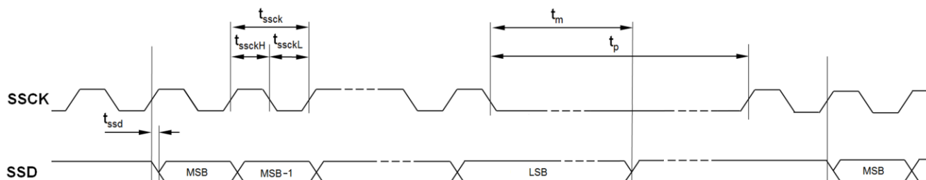
Figure 15: SSI Timing
