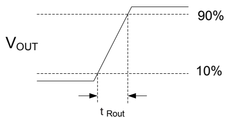
Figure 5. Output Voltage Rise and Fall Times
