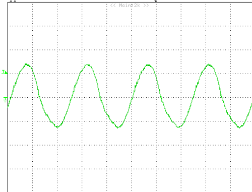
Figure 10: Input Terminal Ripple Current, i_c , at full rated output current and nominal input voltage with 12\mu H source impedance and 33\mu F electrolytic capacitor ( 200 \text{ mA/div} , 1\mu s/div )
