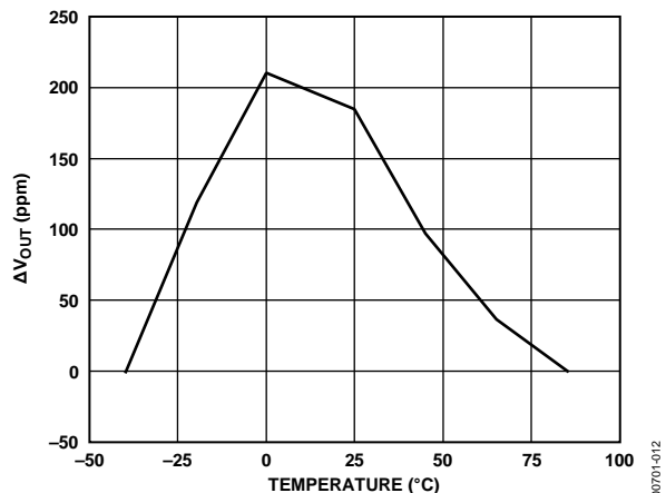
Figure 12. Residual Drift Error
