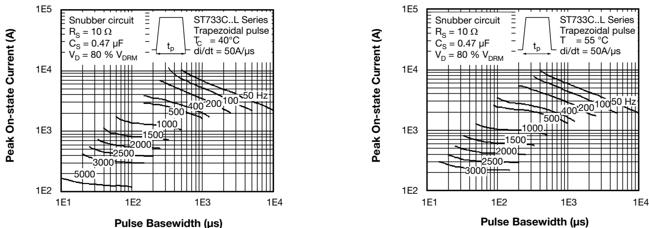
Fig. 15 - Frequency Characteristics
